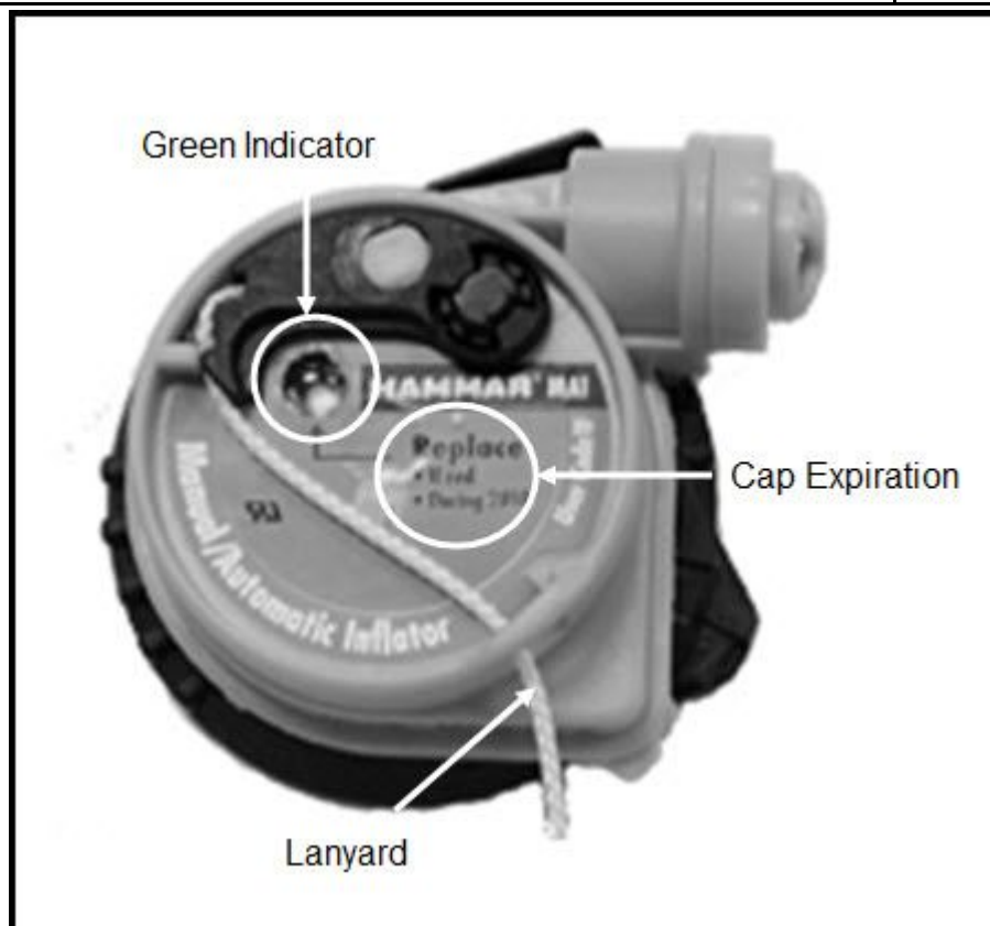
INFLATOR ASSEMBLY Figure 7
