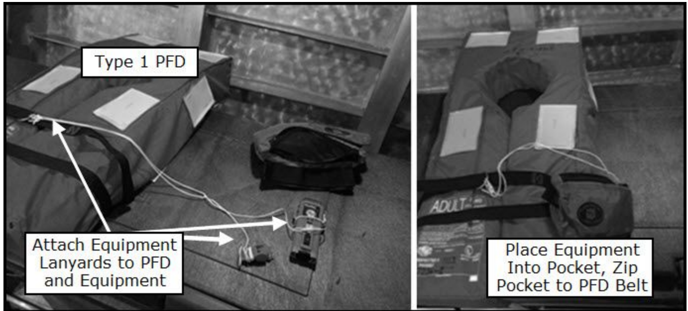
EQUIPMENT POUCH ON TYPE I PFD
